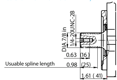
R Splined shaft 7/8 in 13T 16/32 DP 1)
