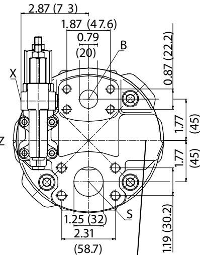
Valve mounting for counter clockwise rotation
