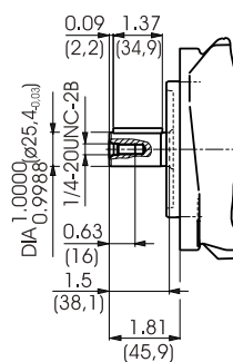
K Parallel with key ISO 3019-1 25-1
