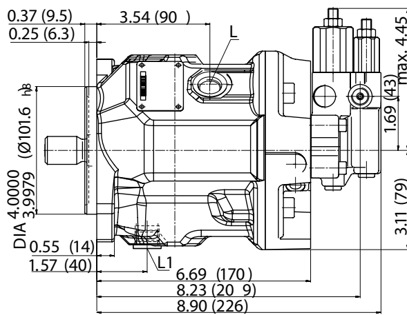
Port plate 61/11
