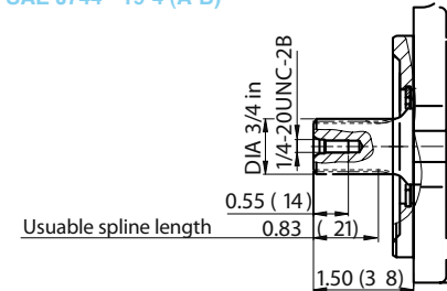
W Splined Shaft 3/4 in 11T 16/32 DP 1) SAE J744 - 19-4 (A-B)
