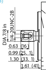
S Splined shaft 7/8 in 13T 16/32 DP 1) SAE J744- 22-4 (B)
