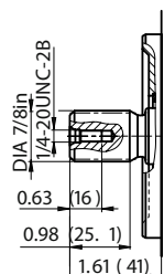
U Splined shaft 7/8 in 13T 16/32 DP SAE J744 - 22-4 (B)
