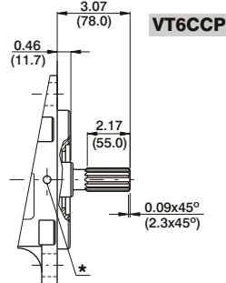
Shaft code 6 non SAE splined shaft Class 1-J498b 12/24 dp. 14 teeth 30° pressure angle Flat root side fit
